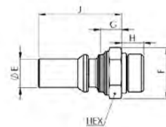
Figure 4 Male ORB ISO 11926-3
