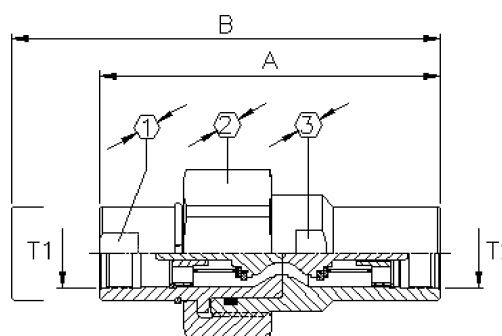
Connected Coupling
