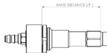
Figure 3 Connected
