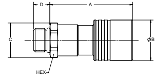
Figure 3 Male ORB
