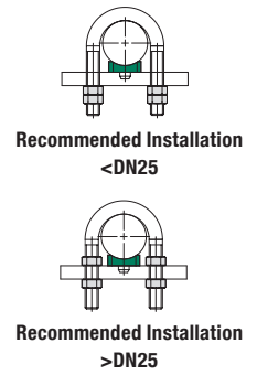
Round Steel U-Bolt (type RB) with Plastic Pipe Saddle (type RUK)
